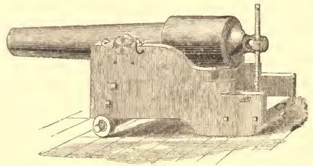
FIG. 13.—Parrott Gun.
